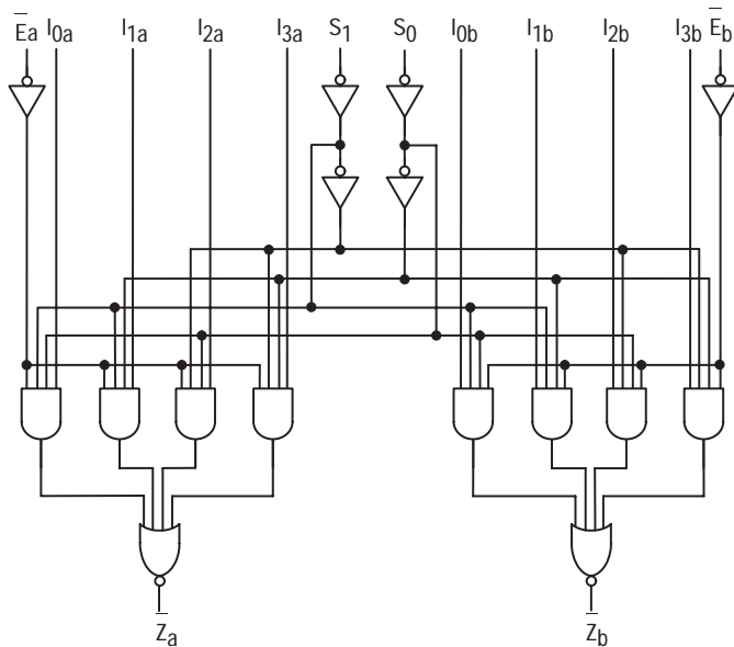
LOGIC DIAGRAM
