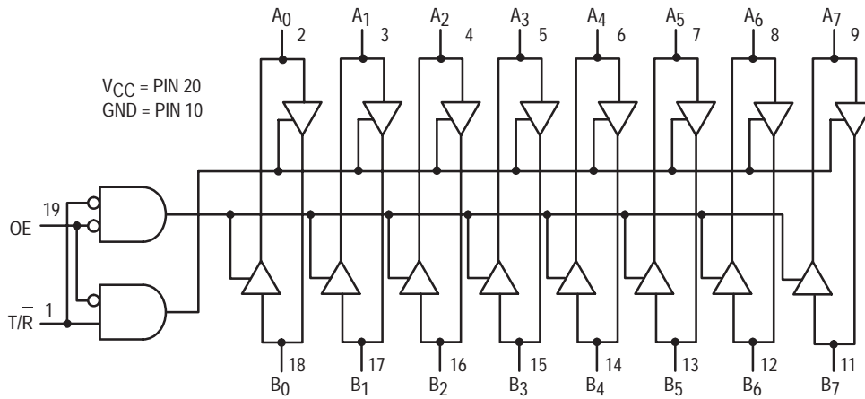
LOGIC DIAGRAM
