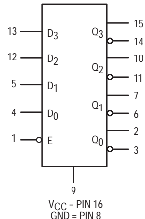
LOGIC SYMBOL
