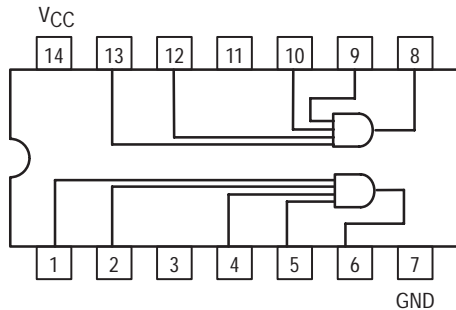
CONNECTION DIAGRAM
